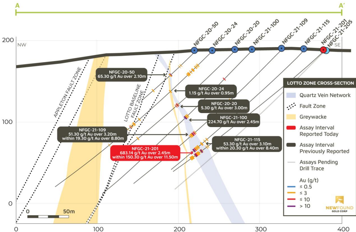
Queensway Project – Cross Section of Current Drilling Program (Lotto Zone – March 23, 2021)
