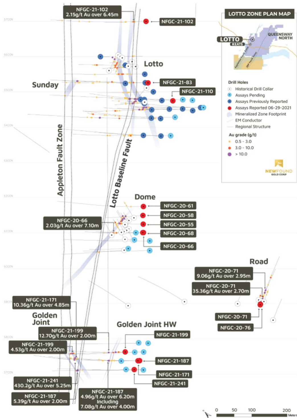
Queensway Project –Golden Joint to Lotto Corridor Map (July 5, 2021)
