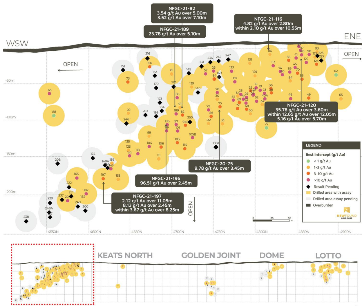
Queensway Project – Long Section of Drilling Program (Keats Zone – May 21, 2021)
