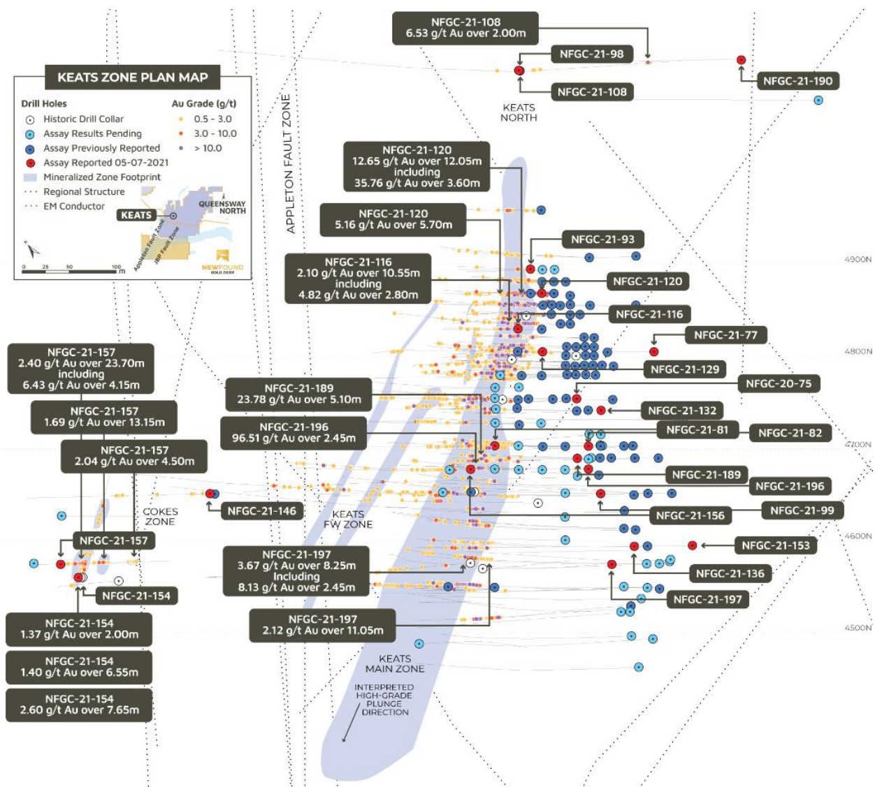
Queensway Project – Plan Map of Drilling Program (Keats/Cokes Zone - July 5, 2021)
